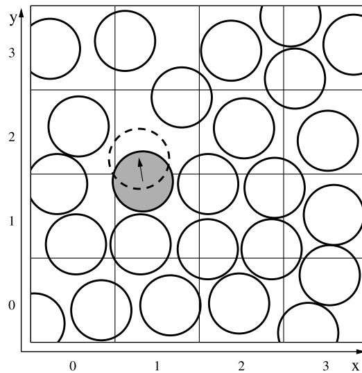
Fig. 1. In a serial hard disk simulation, each trial move typically consists of the following: (i) Select a single disk at random, (ii) apply a random displacement to it, and (iii) accept the move if it generates no overlaps. The cell list enables O(1) overlap checks by limiting the search space to only nine local cells. A sweep is defined as N consecutive trial moves, where N is the number of disks in the simulation.
